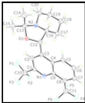
Fig. 1. The molecular structure of (I) showing the atom-labelling scheme and displacement ellipsoids at the 50% probability level.
