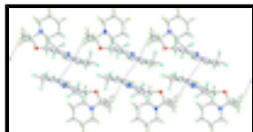
Fig. 2. A view of a supramolecular chain in (I) aligned along the a axis. The C–H \cdots\pi and \pi – \pi interactions are shown as brown and purple dashed lines, respectively. Colour code: F, cyan; O, red; N, blue; C, grey; and H, green.
